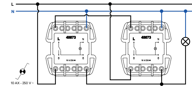
Two-way Switch with Pilot Lamp
