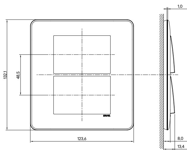
Ref. 41926 T - 3+3 Modules (Crystal)
