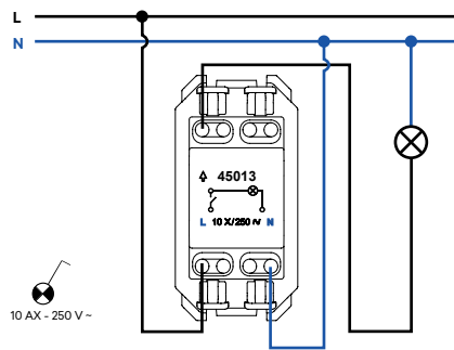
Single Pole Switch with Pilot Lamp
