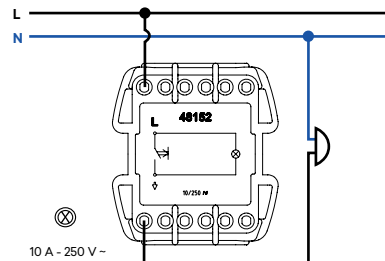
Rocker Push-button with Orienting Light 250 V ~
