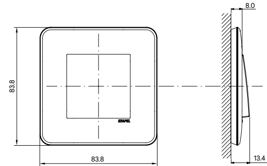
Ref. 42920 T - Double (Croma)
