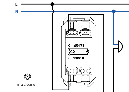
Rocker Push-button with Orienting Light with Symbol
