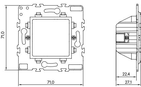
Ref. 42994 - Fixing Adapter with Claws
