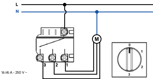
Rotary Switch 4 Positions
