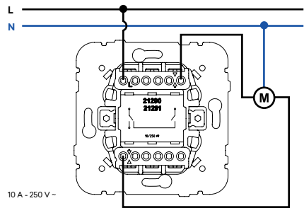
Venetian Switch | Venetian Switch with Mechanical Blockage
