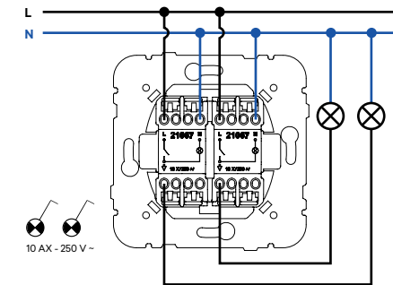
Two Circuits Switch with Pilot Lamp
