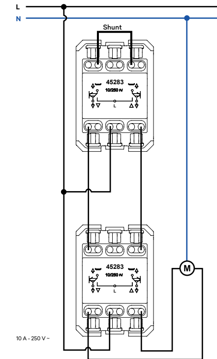
Venetian Double Push-button for Multiple Points Blinds Control (Control from 2 or several points)
