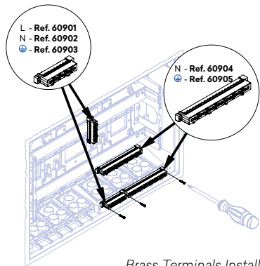
Brass Terminals Installation
