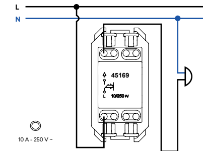
Rocker Push-button with Symbol
