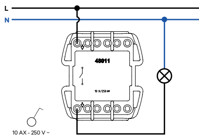
Single Pole Switch
