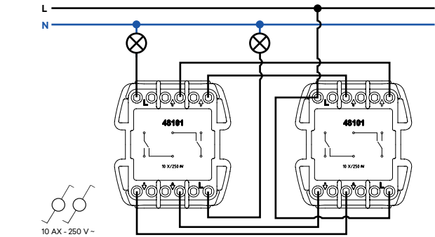
Double Two-way Switch
