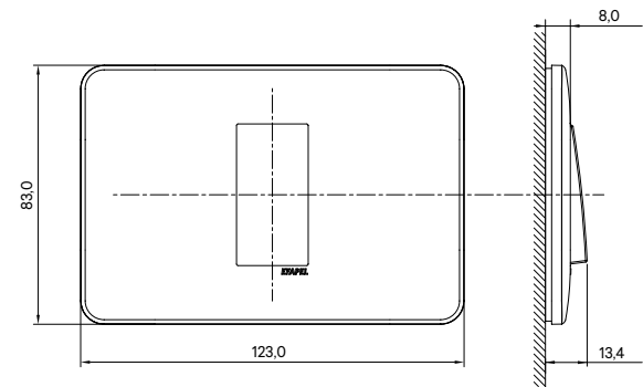
Ref. 41914 T - 2 Modules (Standard, Aquarella)
