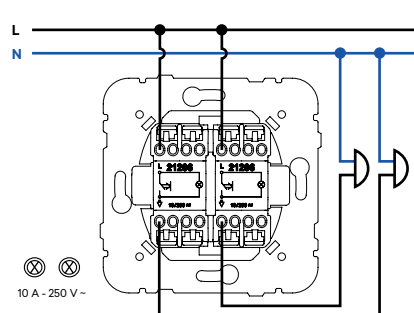
Double Rocker Push-button with Orienting Light 250 V ~
