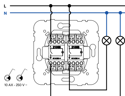
Two Circuits Switch with Pilot Lamp
