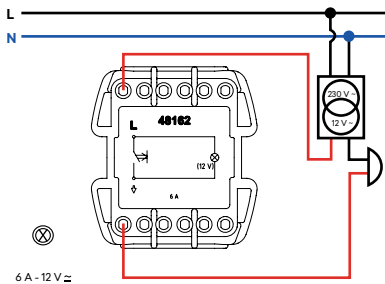
Rocker Push-button with Orienting Light 12 V =
